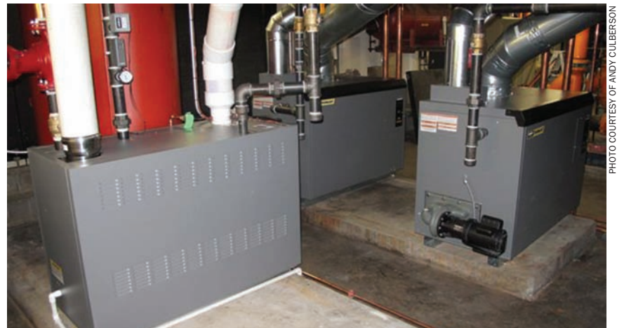
The new hydronics system at the Lutheran Home of Concord Reserve features one 850-MBH cold-start condensing boiler and two 1,000-MBH sealed-combustion, fan-induced, two-stage boilers.
